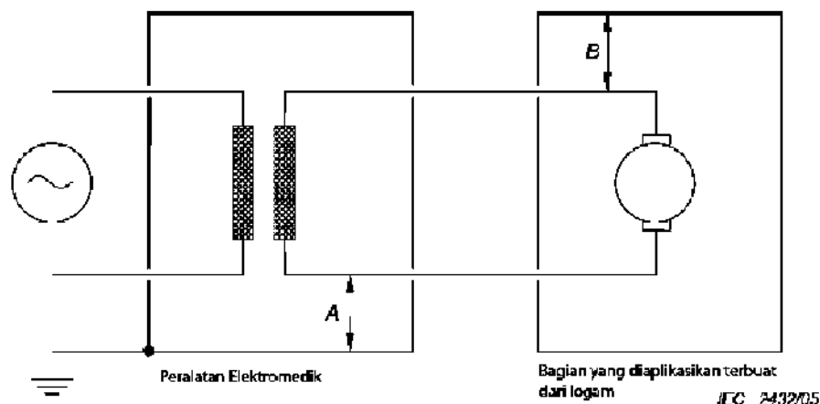
Gambar A.10 – Sirkuit floating
