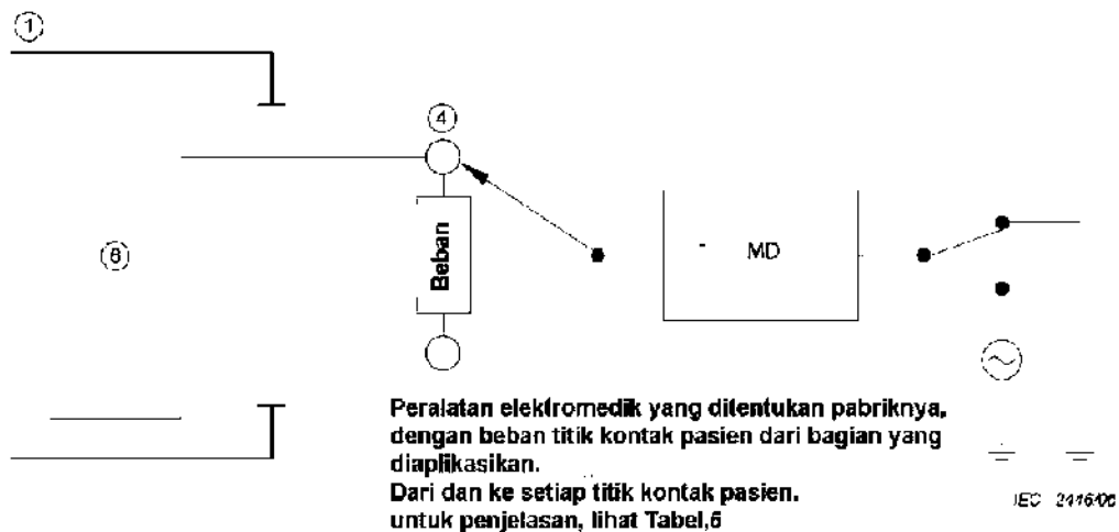
Gambar E.4 – Patient auxiliary current
