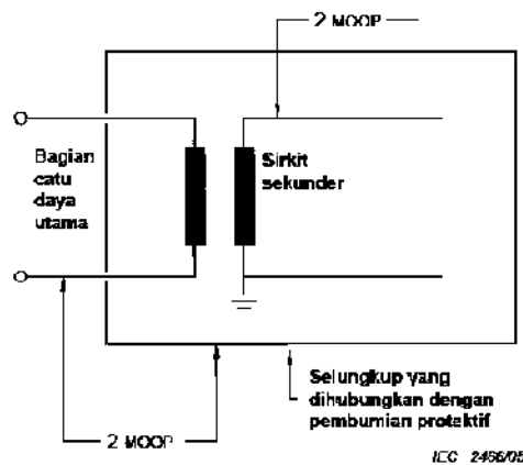
Gambar J.2 – Isolasi contoh 2
