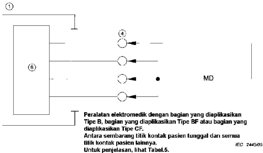
Gambar E.4 – Patient auxiliary current
