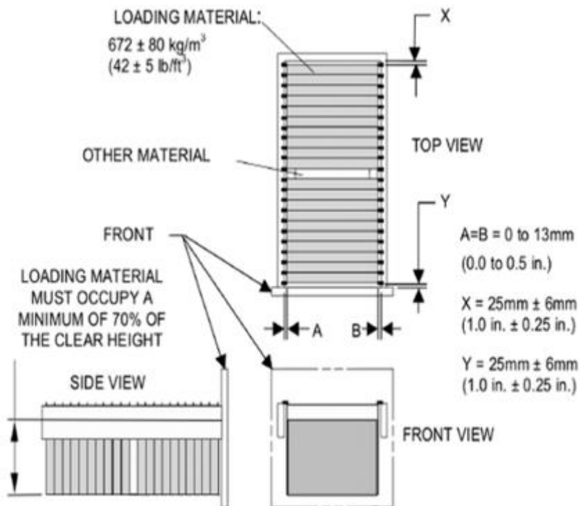
Figure 3c - Loading Configuration for Extendible Elements (Deeper than Wide) without Bottoms
