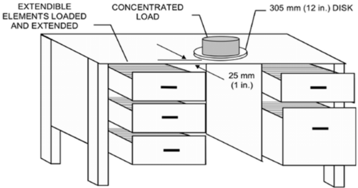
Figure 5a – Concentrated Load Test for Primary Surfaces
