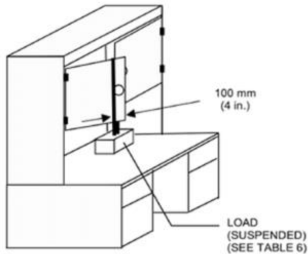
Figure 17a - Strength Test for Vertically Hinged Doors, Bi-fold Doors, and Vertically Receding Doors
