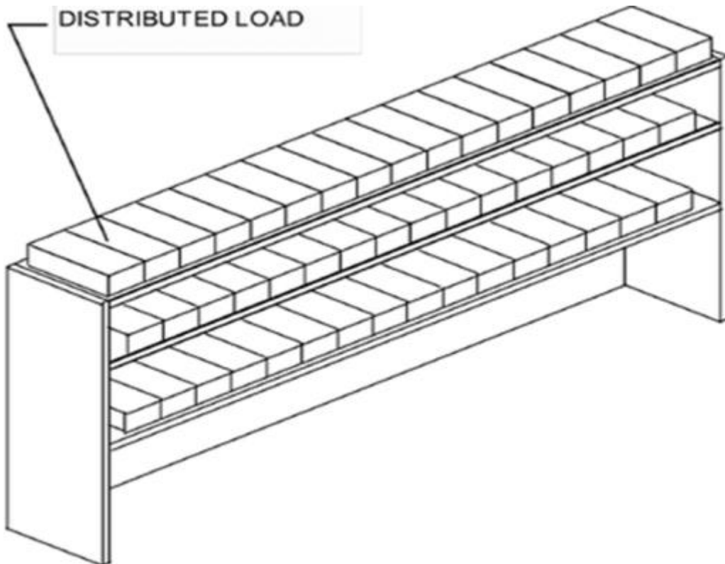
Figure 5f - Distributed Load Tests for Secondary Surfaces
