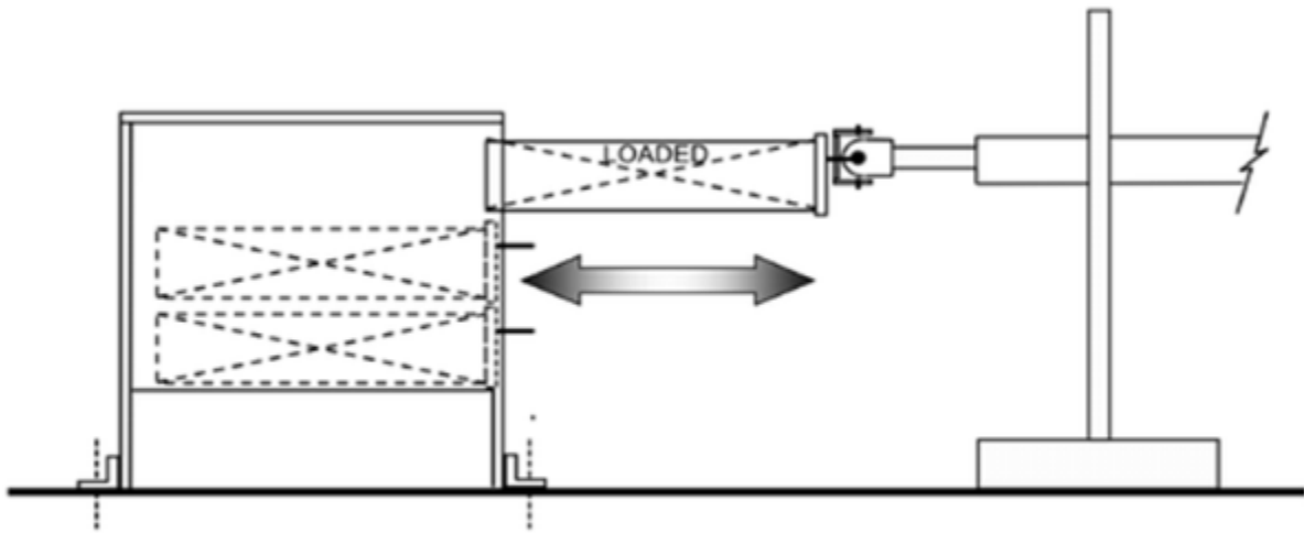
Figure 10 - Extensible Element Cycle Test
