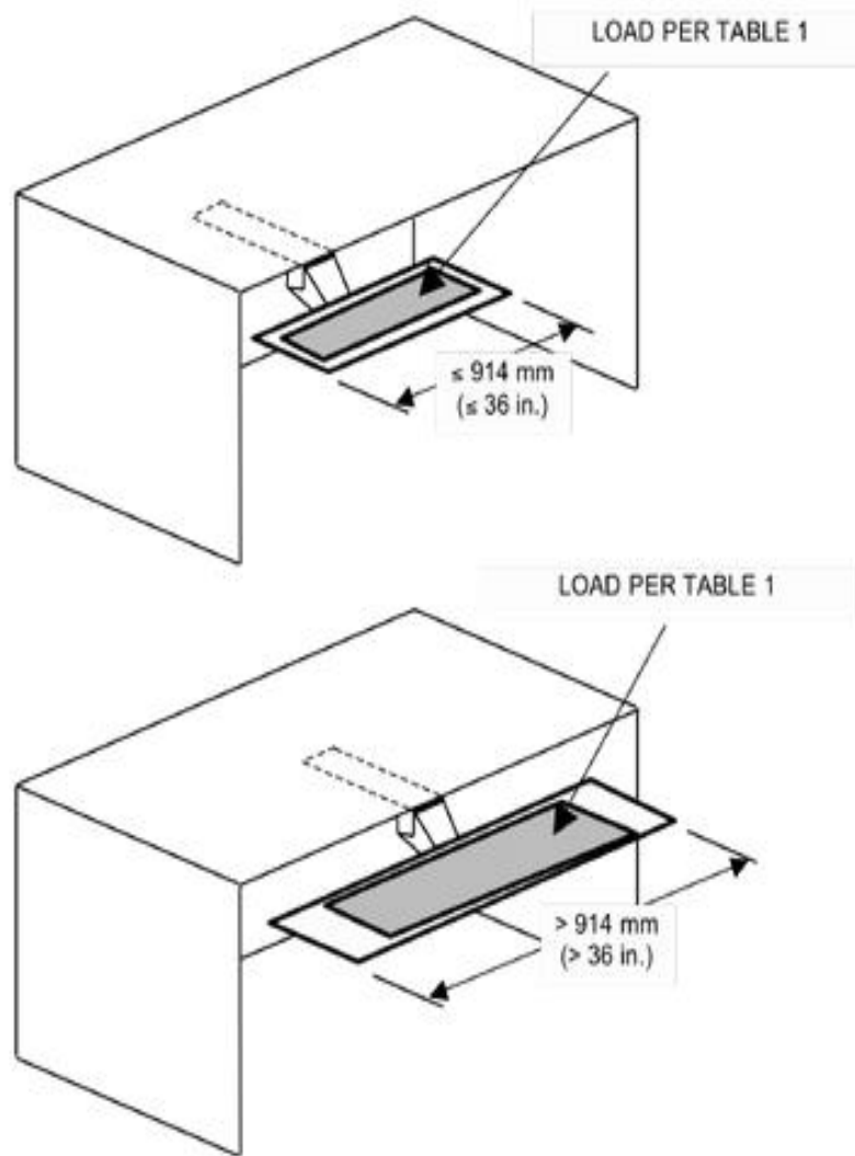
Figure 5h - Distributed Load Tests for Adjustable Keyboard Supports
