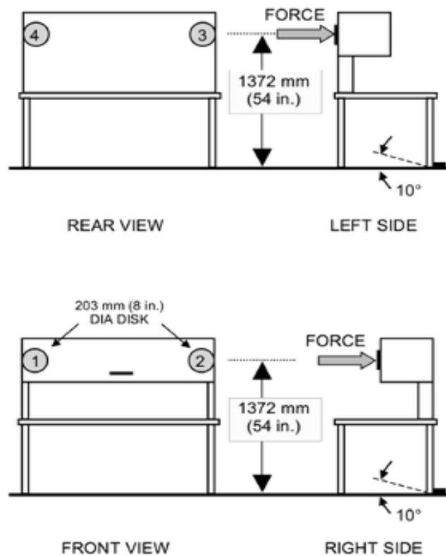
Figure 4e - Force Stability Test for Tall Desk/Table Products
