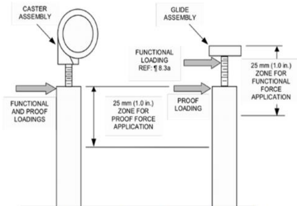
Figure 8 Continued - Leg Strength Test – Typical Load Application
