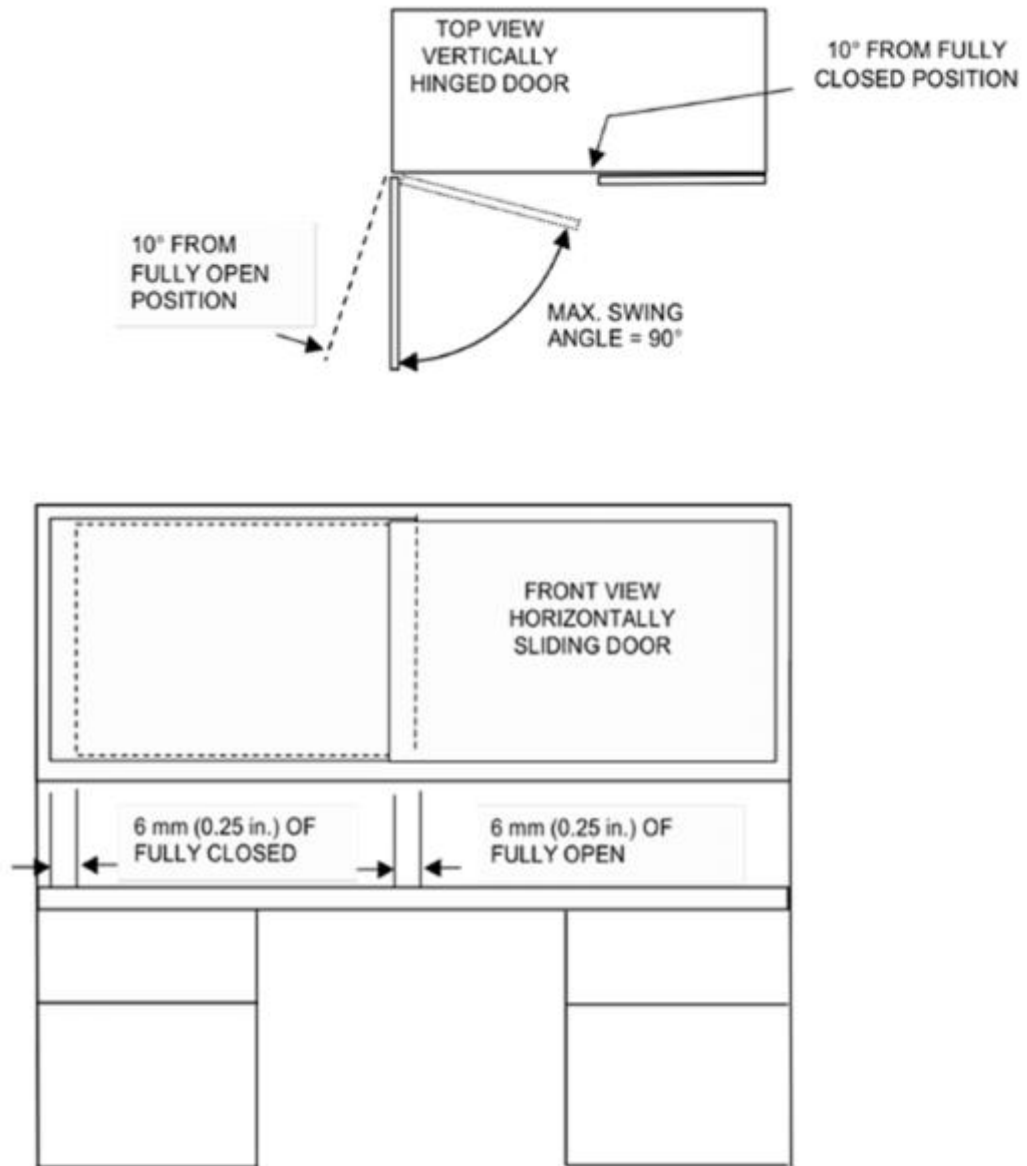
Figure 17e - Wear and Fatigue Test for Hinged, Horizontally Sliding, and Tambour Doors
