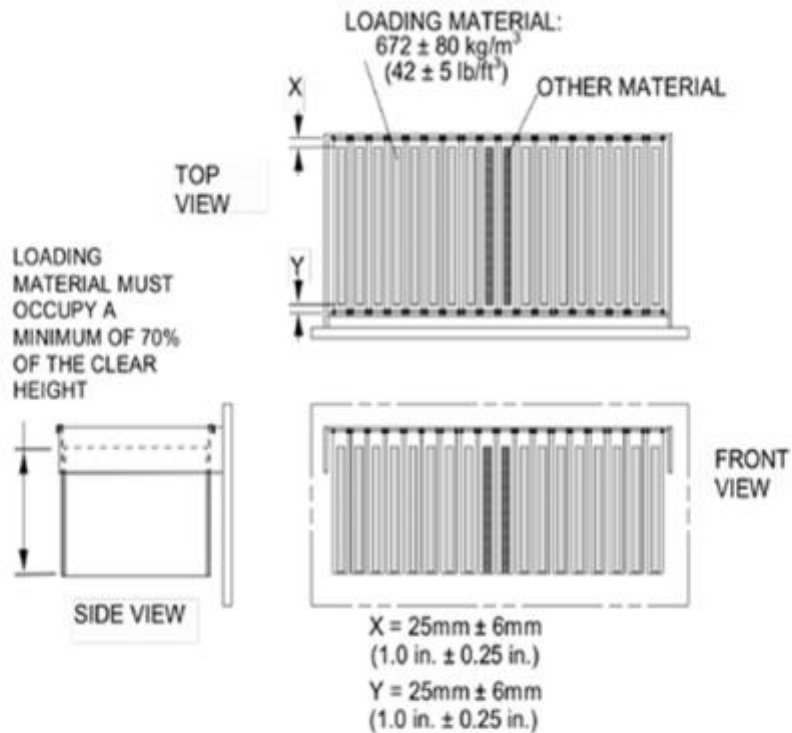
Figure 3d - Loading Configuration for Extendible Elements (Wider than Deep) Without Bottoms
