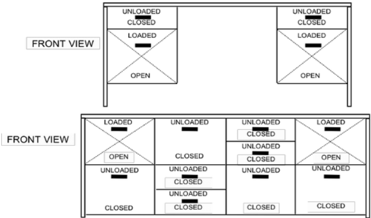
Figure 4a - Stability with Extendible Elements Open
