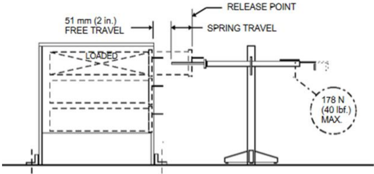
Figure 12 – Extensible Element Rebound Test
