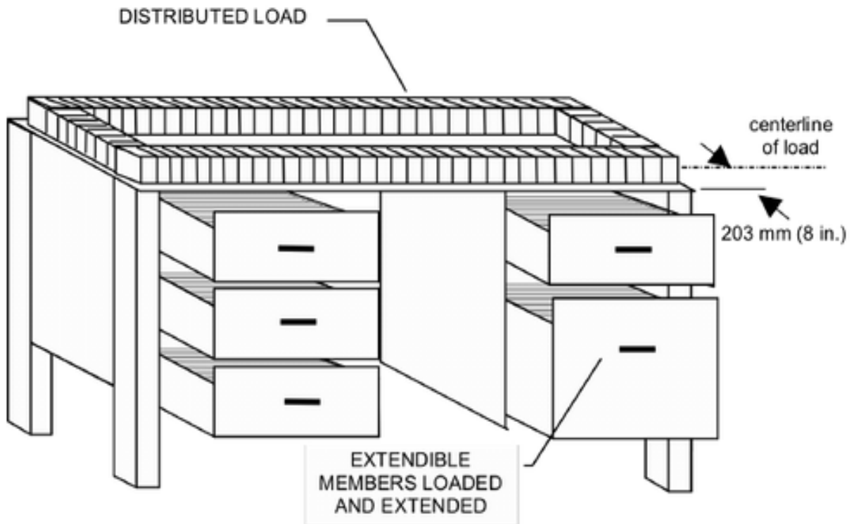
Figure 5e - Distributed Load Tests for Primary Surfaces
