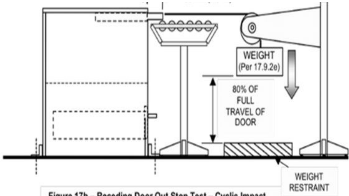
Figure 17h – Receding Door Out Stop Test – Cyclic Impact
