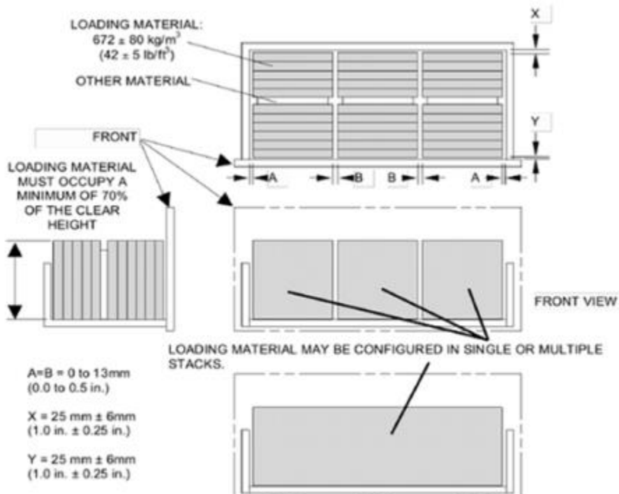
Figure 3b - Loading Configuration for Extendible Elements (Wider than Deep) With Bottoms
