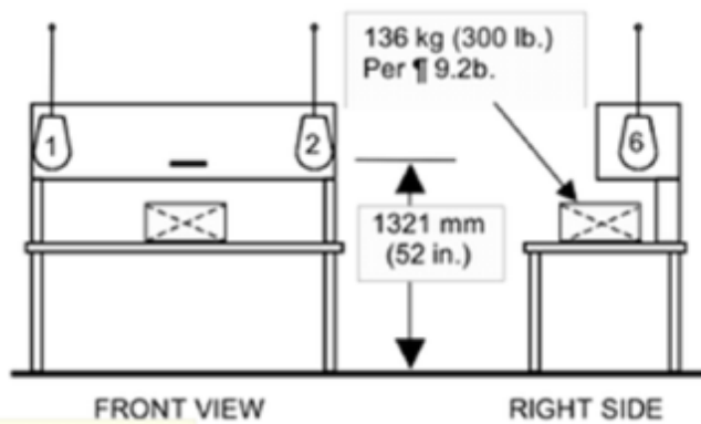
Figure 9 - Disengagement Tests for Tall Desk/Table Products
