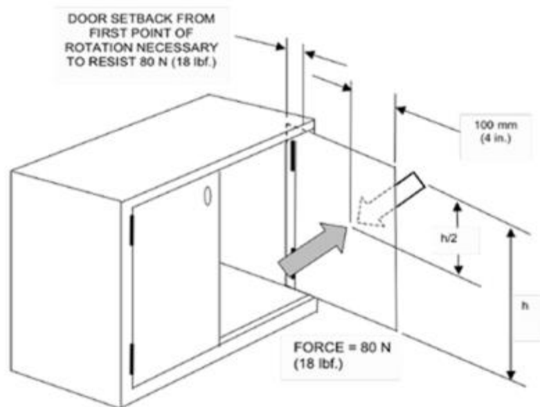
Figure 17c – Vertical Receding Doors Strength Test
