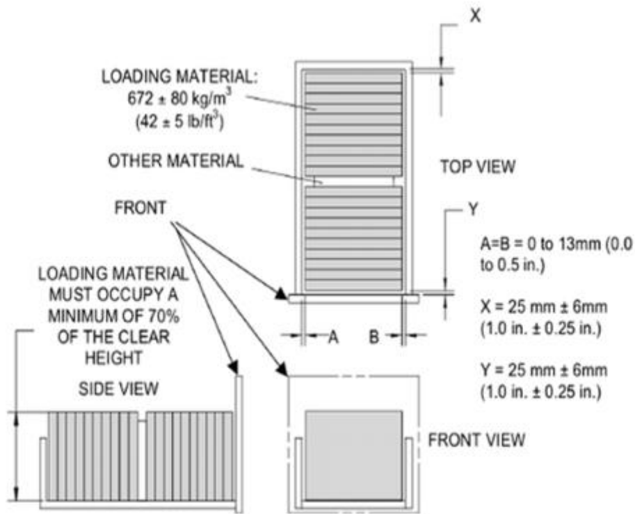
Figure 3a - Loading Configuration for Extendible Elements (Deeper than Wide) with Bottoms
