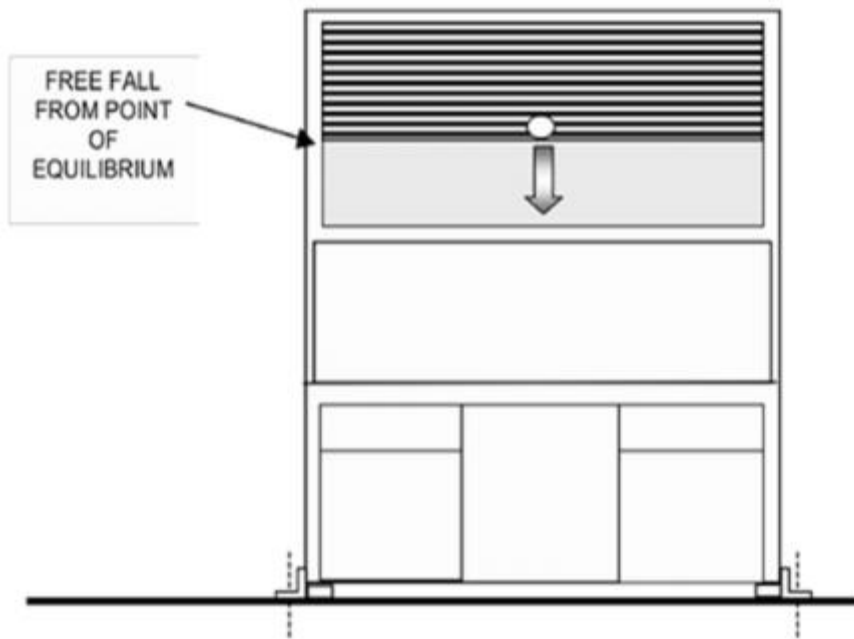
Figure 17L – Slam Test for Doors Which Free Fall Open or Closed
