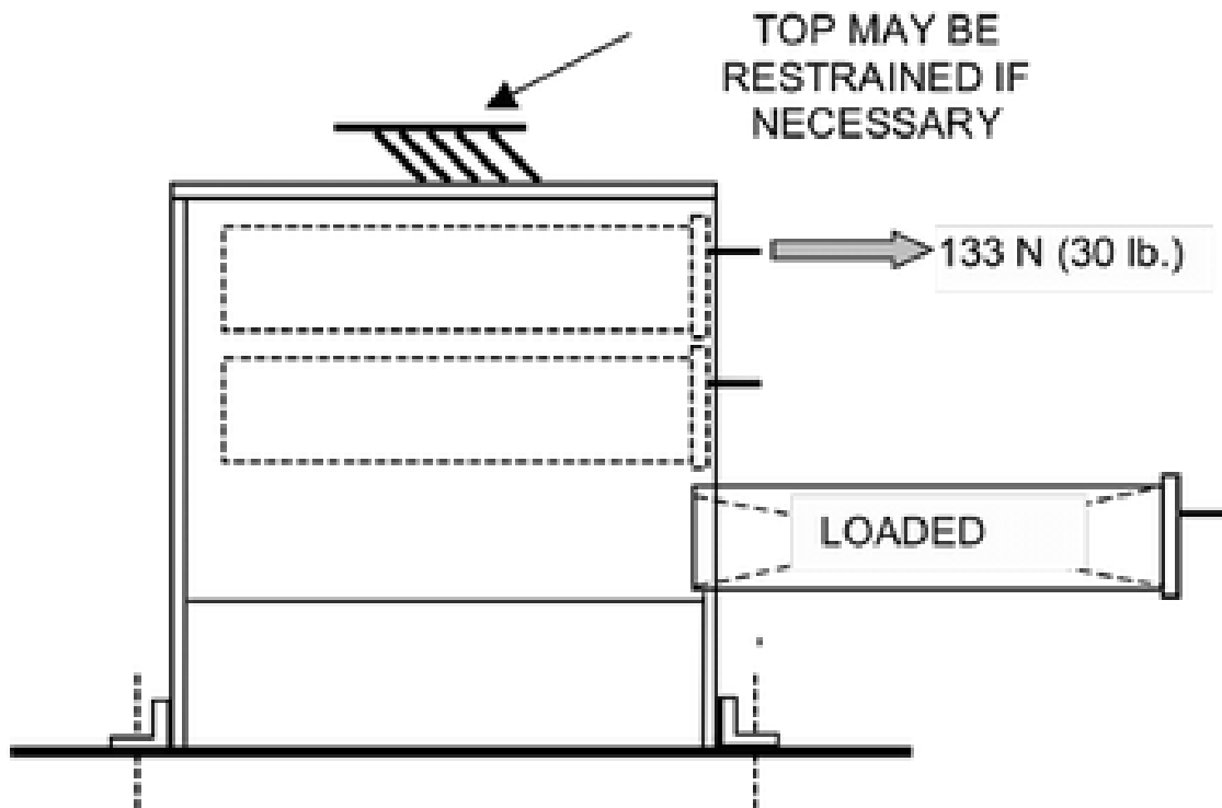
Figure 13 – Interlock Strength Test
