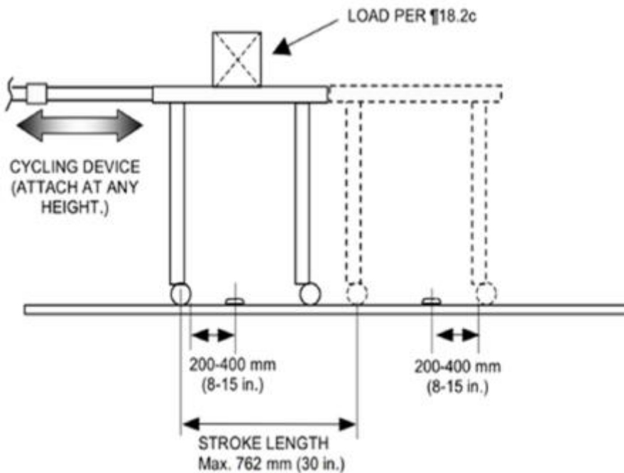
Figure 18 - Durability Test for Desks and Tables with Casters
