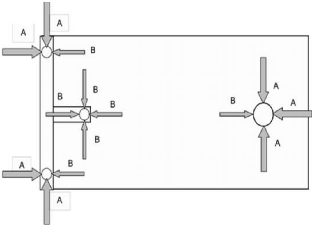
Figure 8 Continued - Leg Strength Test – Typical Configurations
