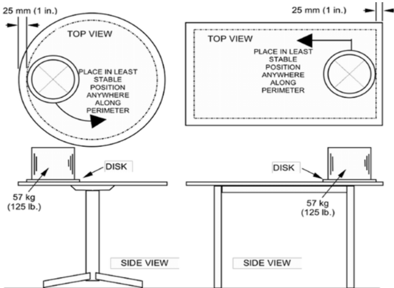
Figure 4b - Stability Under Vertical Load
