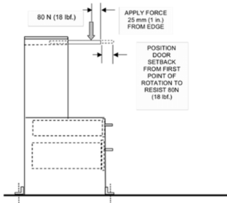
Figure 17d – Horizontal Receding Doors Strength Test
