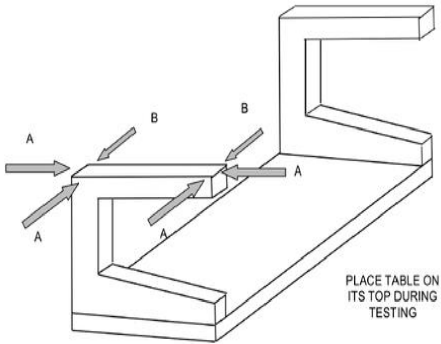
C-LEG TABLES TESTED AS SHOWN ABOVE
