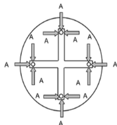
CROSS SLAB LEGS TESTED AS SHOWN ABOVE
