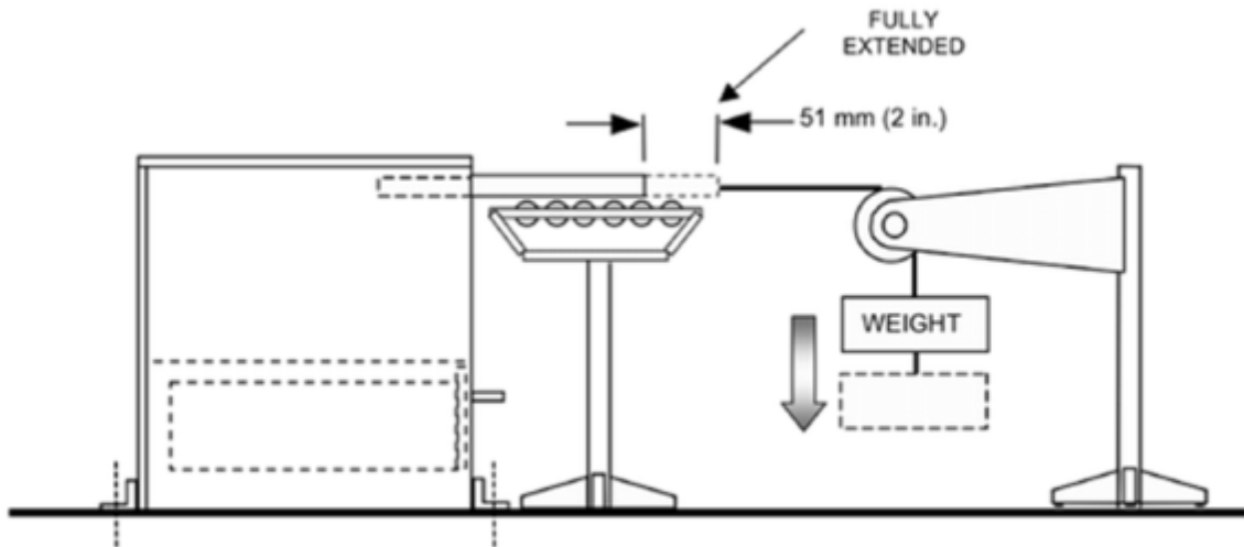
Figure 17i – Receding Door Out Stop Test – Cyclic Durability
