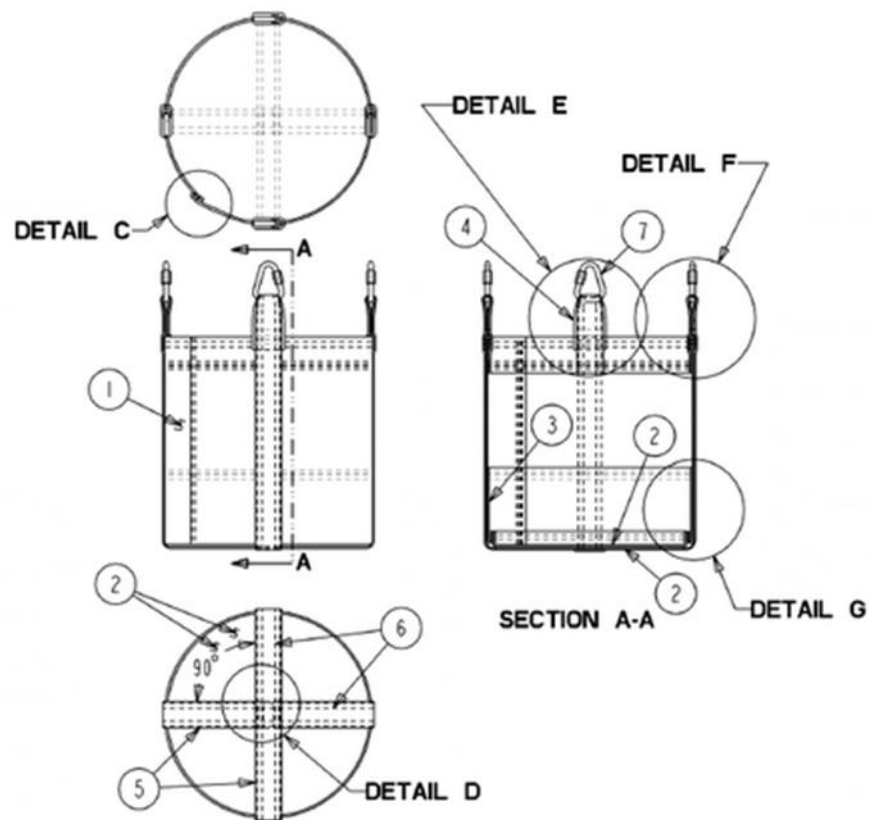
Appendix A (Continued) – Load Ease Test Bag – Typical Construction
