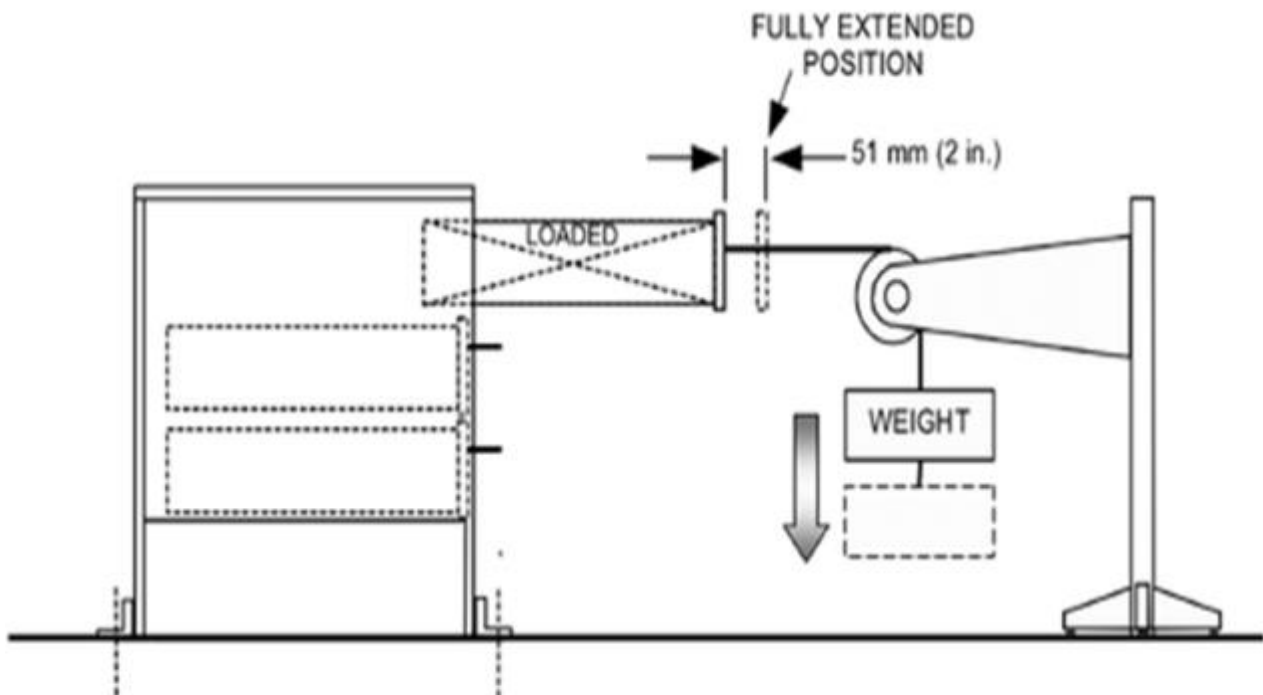
Figure 11b – Extendible Element Retention Durability Test
