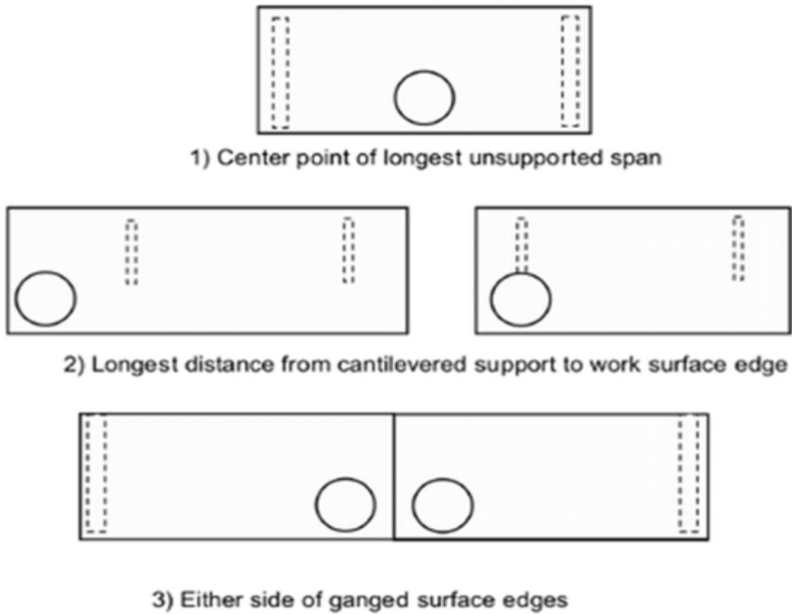
Figure 5b - Top View of Placement of Concentrated Load(s)
