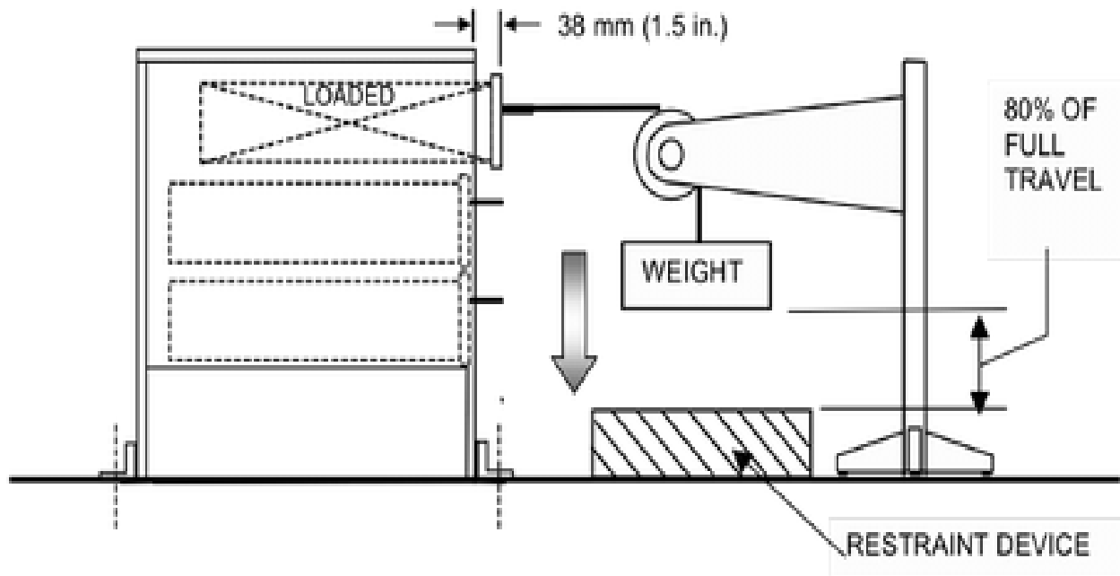
Figure 11a – Extendible Element Retention Impact Test
