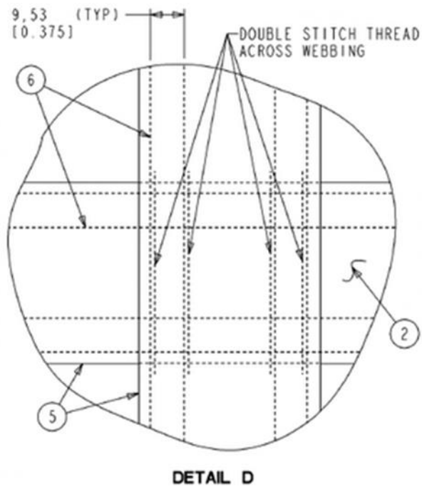
Appendix A (Continued) – Load Ease Test Bag – Typical Construction
